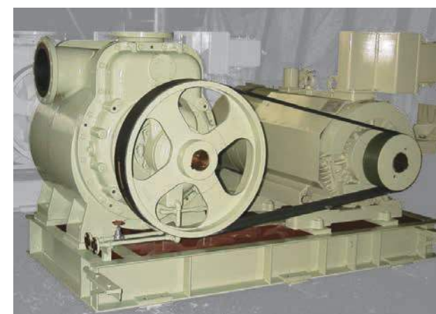
Flue Gas Desulfurization Vacuum Pump 250V690V, 90 kW × 500 min -1 140 m 3 /min × -67 kPa (G)
