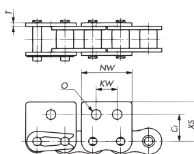
WSK1, WSK2 Attachment
