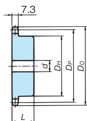
Hub without groove (13 and over)
