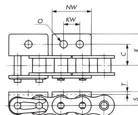
WSA1, WSA2 Attachment
