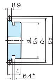
Hub with groove (10T to 13T)
