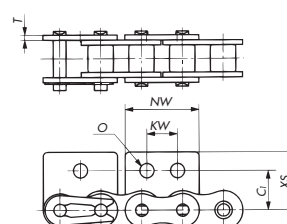
WSA1, WSA2 Attachment
