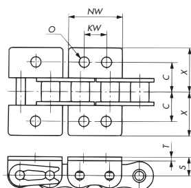
WK1, WK2 Attachment
