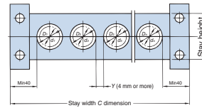
Relationship between standard stay width (C) and bending radius (R)
